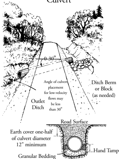
Typical Upland Cross-Drainage Culvert
